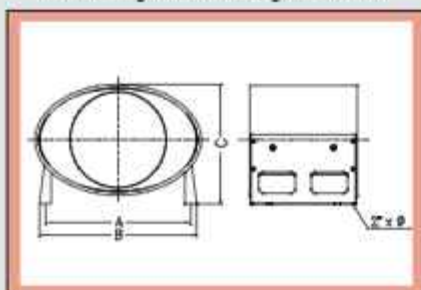
Mounting Feet & Hanger - IJB-O
