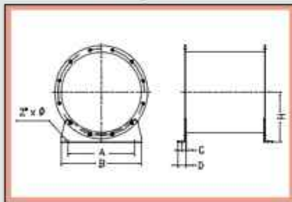
Mounting Feet - IJB
